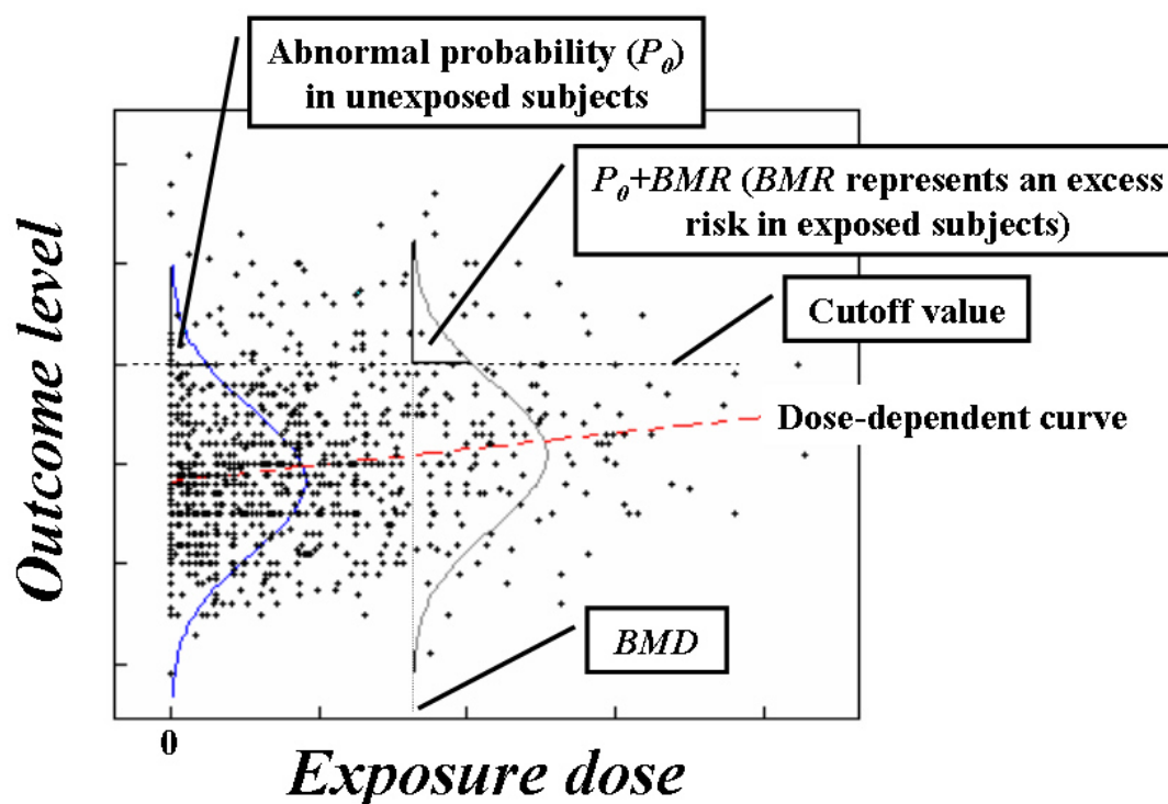
Fig. 1 Hypothetical dose-effect (response) relation illustrating the concepts of the benchmark dose method. The dose-dependent curve indicates that when the exposure dose increases, so does the expected outcome level. The distribution of outcome levels in unexposed subjects is shown at 0 of the x-axis. Outcome levels above the cutoff value are considered abnormal. The risk of an abnormal response in unexposed subjects is P_0 . At the BMD, the distribution has been translated upward and the risk of an abnormal response has increased to P_0+BMR . The BMDL (the statistical 95% lower bound of the BMD) is placed somewhere between zero and the estimated BMD, depending on the amount of information in the study.
